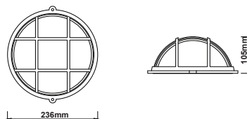
Dimension ( mm )
